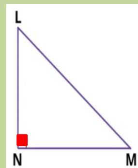
Triangle rectangle LMN
